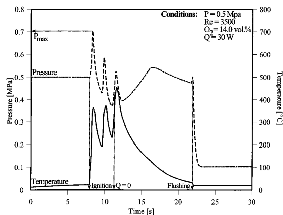
Figure A3. Pressure and temperature increase in an open tube.
