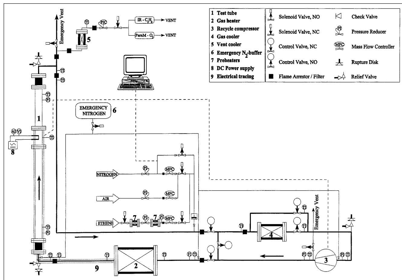
Figure 1. Test installation.
